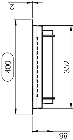
Vorderansicht / Front view Variante A / Version A
